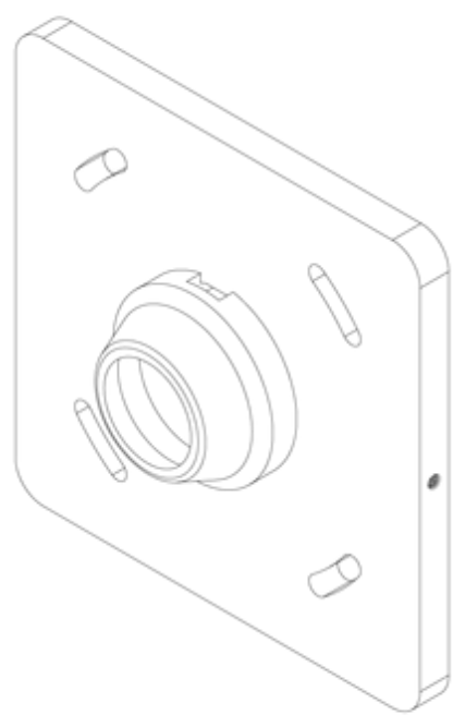
A. Mounting Plate (x1) Install Dimensions: 4.75" x 4.75"
